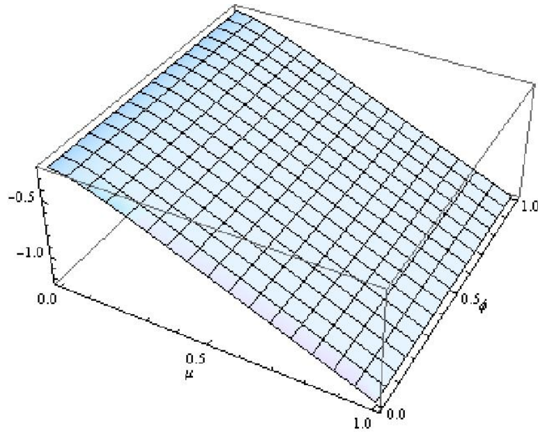
Figure 6: Eigenvalue 1
