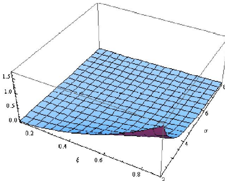
Figure 1: Derivative of \bar{E}_{sym} with respect to \mu
